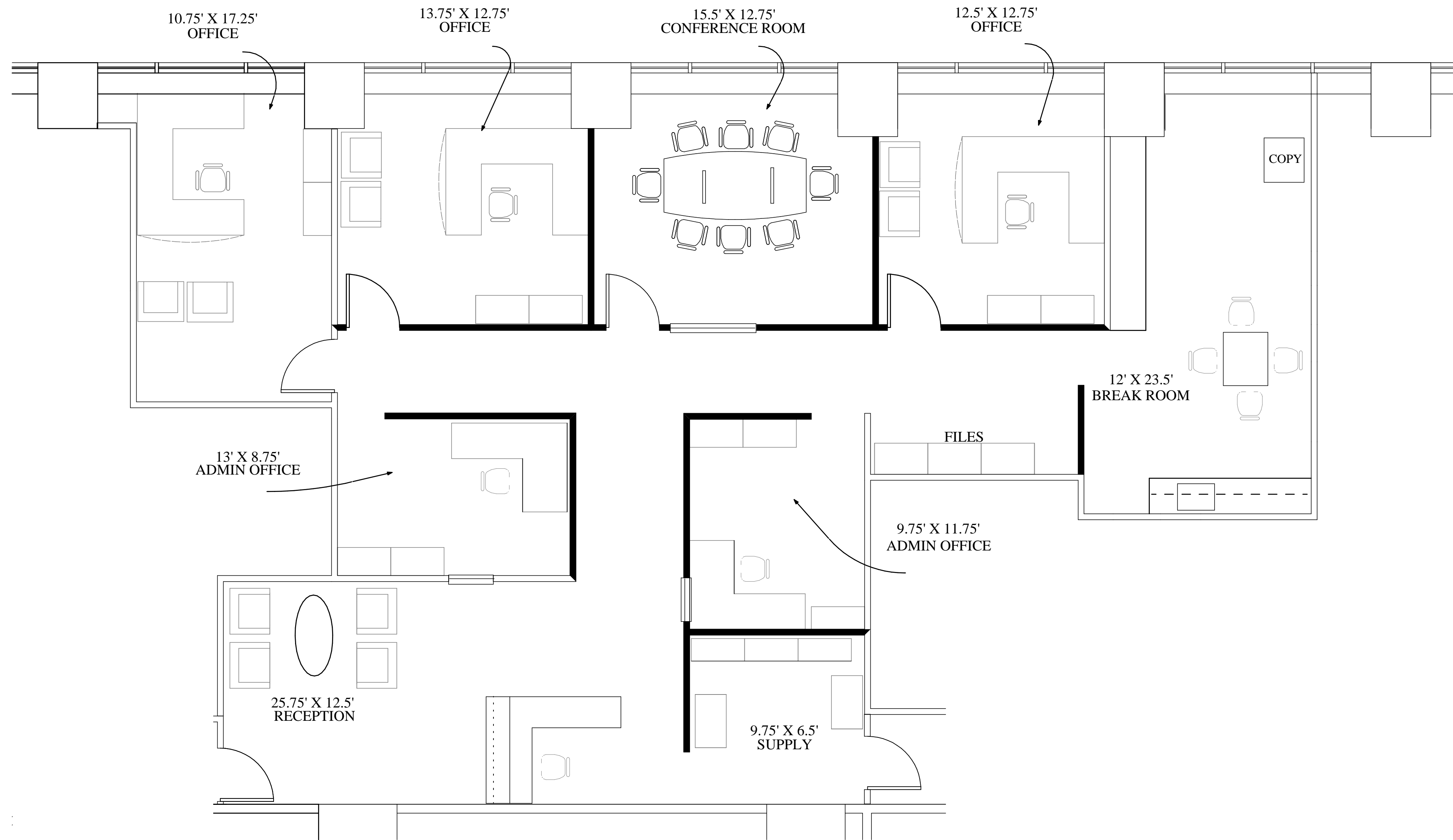
1 SPACE STUDY SS11.4 SCALE: 1/8" = 1'-0"
